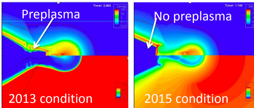
2D hydro dynamic simulation results
