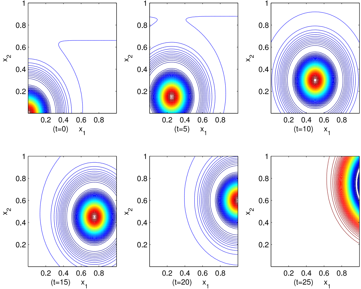
Snapshots with contour plots of the logarithmic density
