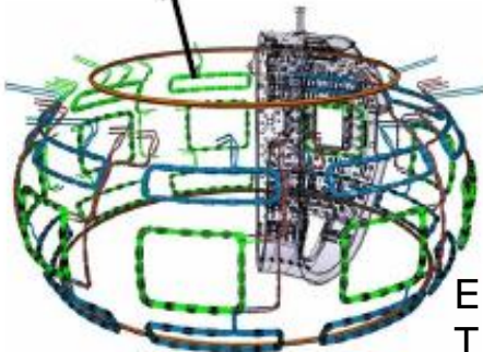
ITER ELM coil (IEC)
