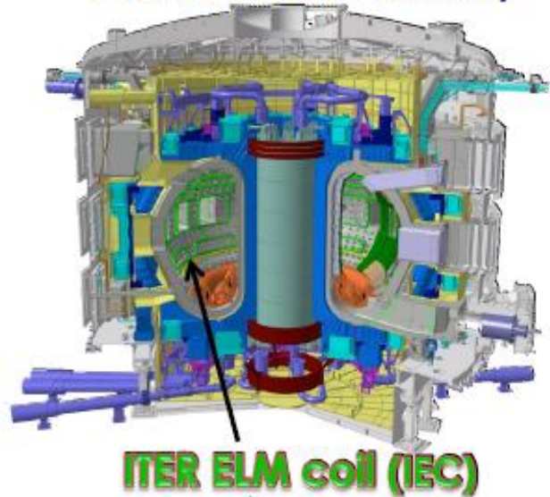
ITER Tokamak Cutaway
