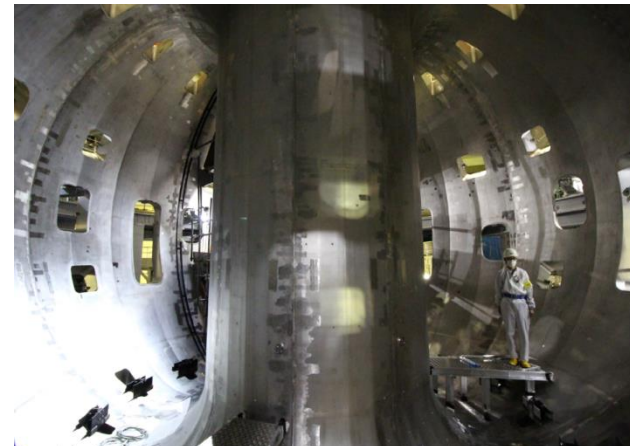
Inside the Vacuum Vessel
