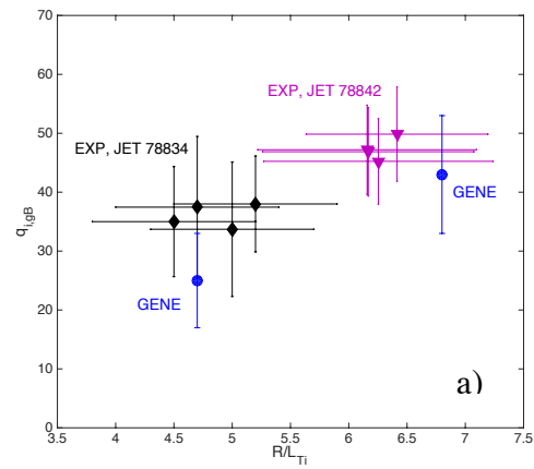
FIG.8 (a) q_{i,gB} vs R/L_{Ti} . Experimental flux of the ICRH case (black) and of the ICRH+NBI case (purple) and GENE TEM/ITG flux for both cases (blue).
