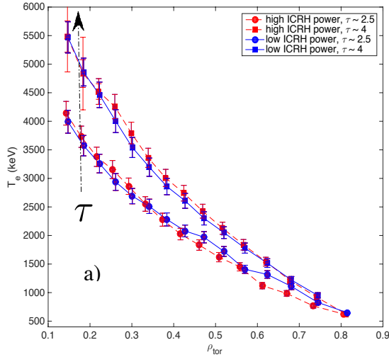
FIG. 6. a) Temperature profiles for shots with fixed s , s/q , n_e and with high and low ICRH power to electrons and different \tau values as shown in b)
