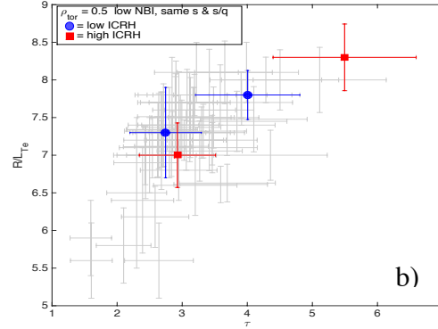
FIG. 6. a) Temperature profiles for shots with fixed s , s/q , n_e and with high and low ICRH power to electrons and different \tau values as shown in b)
