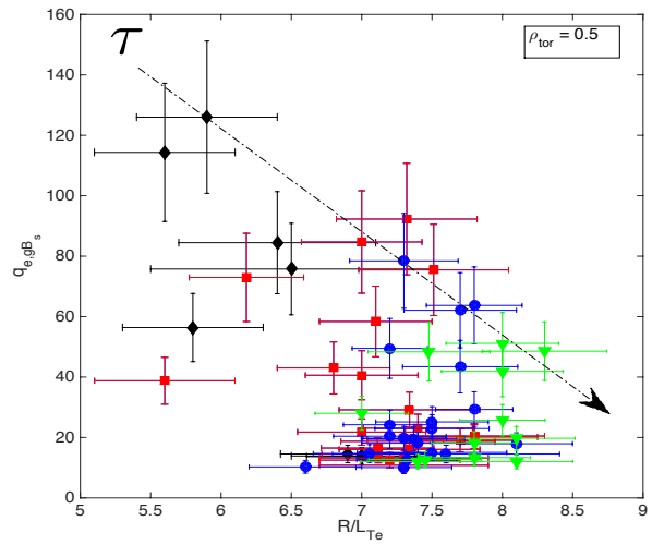
FIG.5. Normalized electron heat flux q_{e,gB} vs R/L_{Te} at \rho_{tor}=0.5 for the same shots as in Fig. 4. Each colour marks a range of \tau values.
