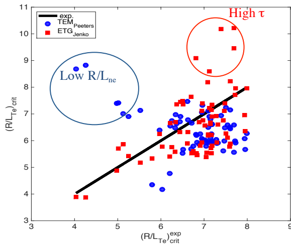
FIG.1. Critical R/L_{Te} calculated with analytical formulae for TEM (blue, from [11]) and ETG (red, from [12]) vs the experimentally derived value in an expanded dataset with respect to that used in [8].
