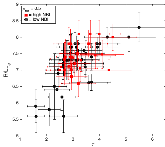
FIG.4. R/L_{Te} vs \tau at \rho_{tor}=0.5 for the same data of Fig.2.
