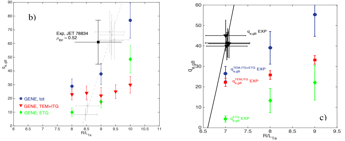
FIG. 8 (b) and (c). q_{e,GB} vs R/L_{Te} . Experimental flux (black/grey), GENE TEM/ITG flux (red), GENE single scale ETG flux (green) and GENE TEM/ITG+ETG flux (blue) for discharges with pure ICRH heating (b) and for discharges with ICRH+NBI heating (c). The black/grey lines indicate the experimental slope (stiffness) of the electron heat flux.
