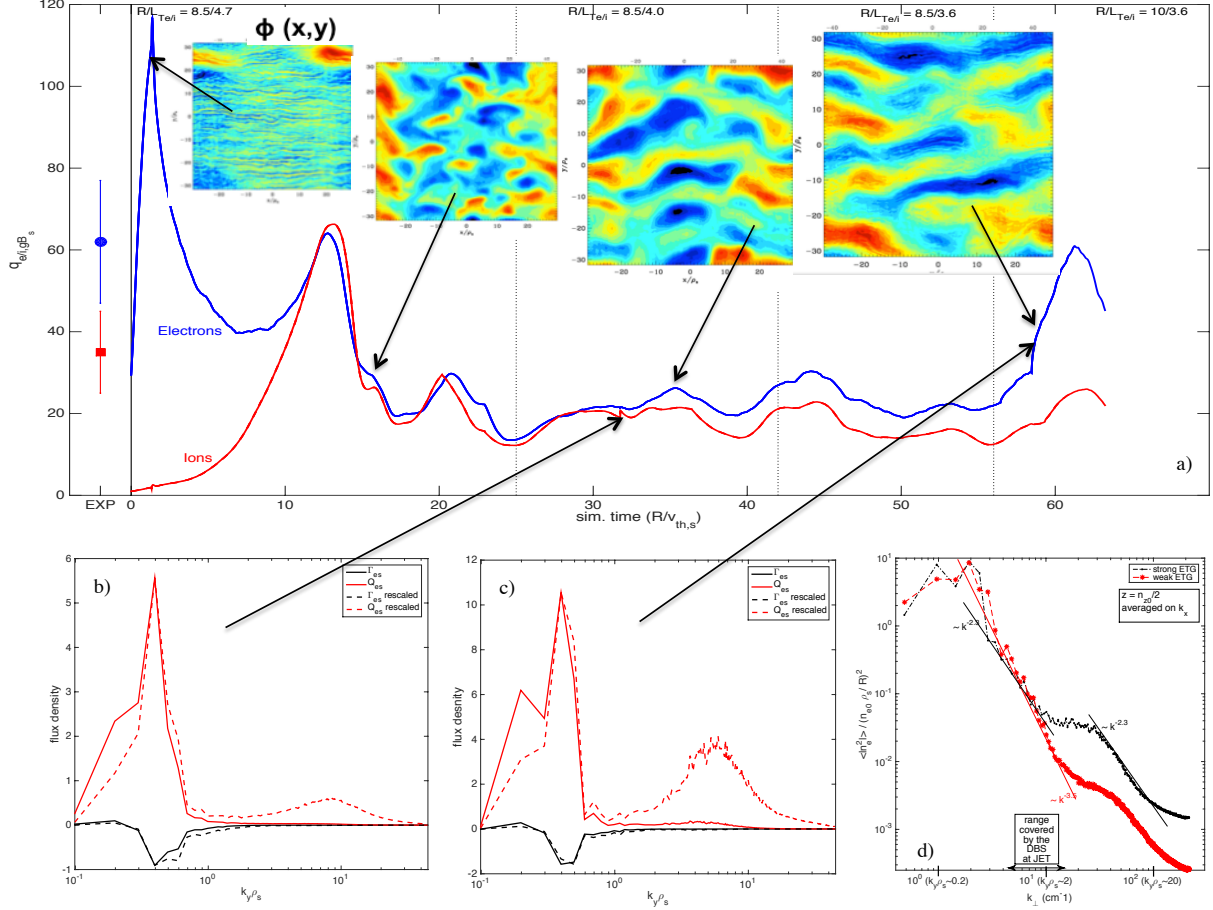
FIG. 9. a) q_{gB} vs simulation time from the multi-scale simulation. The contour-plots of the electrostatic potential is shown for different times. b) & c) Heat and particle flux spectra at two different times: the contribution of ETGs is visible at high k_y . d) Density fluctuation spectra at two different times: when ETGs become more strong the slope at low k_y tend to become lower and a second maximum appears at the ETG peak.
