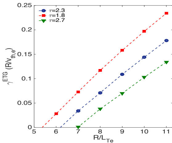
FIG.7: ETG linear growth rates vs R/L_{Te} for different values of \tau .
