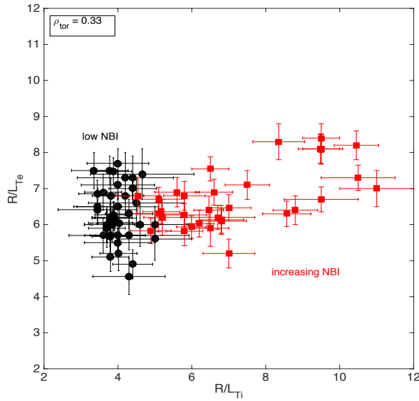
FIG.2. R/L_{Te} vs R/L_{Ti} at \rho_{tor}=0.33 for a series of JET L-mode plasmas with different types of heating.
