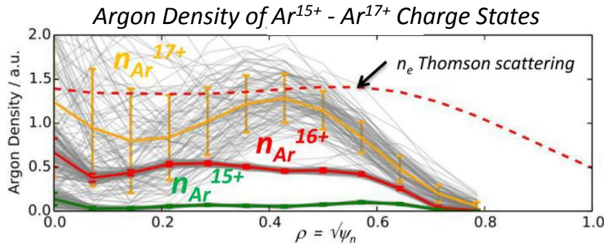
a) nAr16+ Profiles
