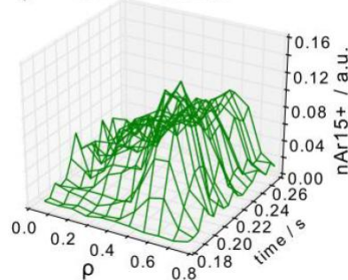
b) nAr15+ Profiles
