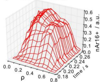
a) nAr16+ Profiles
