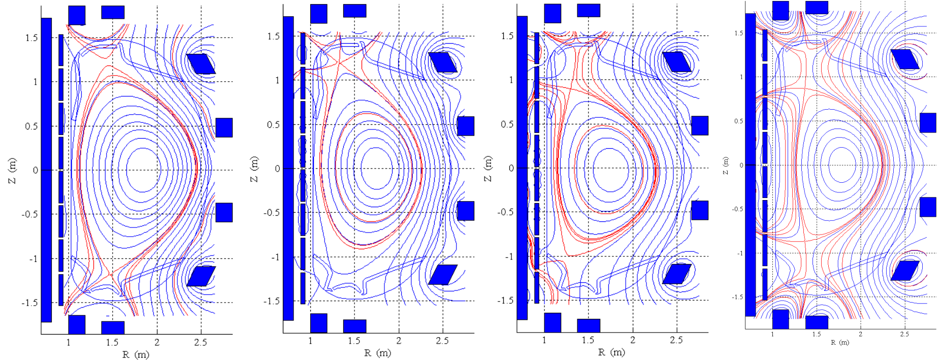
Double null tripod divertor
