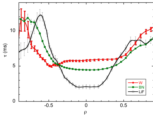
Confinement: radial dependence from local bolometer data
