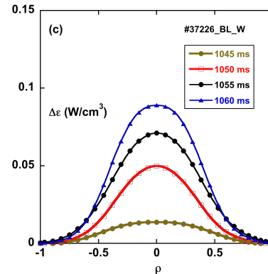
Effect of W injection in bolometer array and n_e(r)
