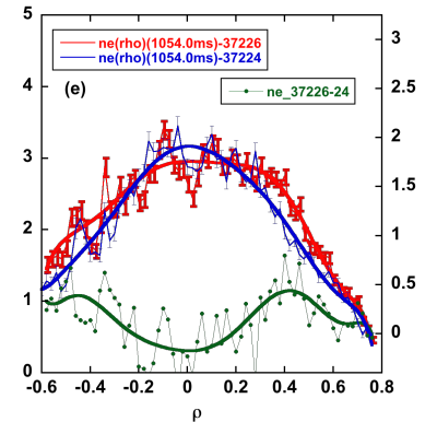
Effect of W injection in bolometer array and n_e(r)
