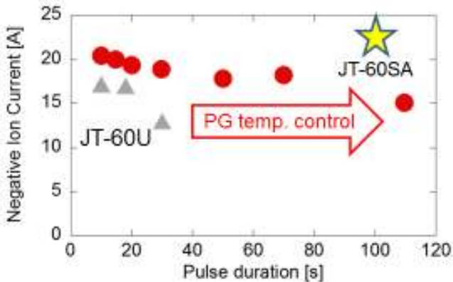
Long pulse beam production 100 s beam production at 15 A
