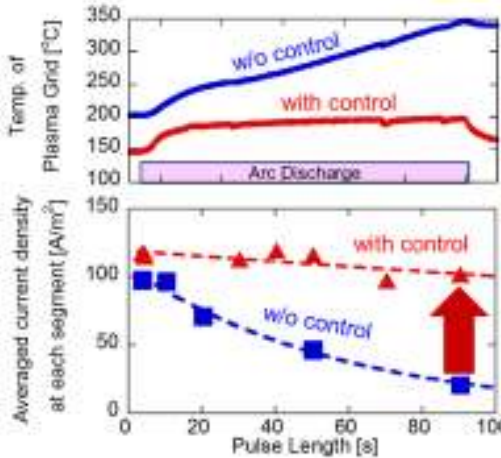
Active control of PG temp.
