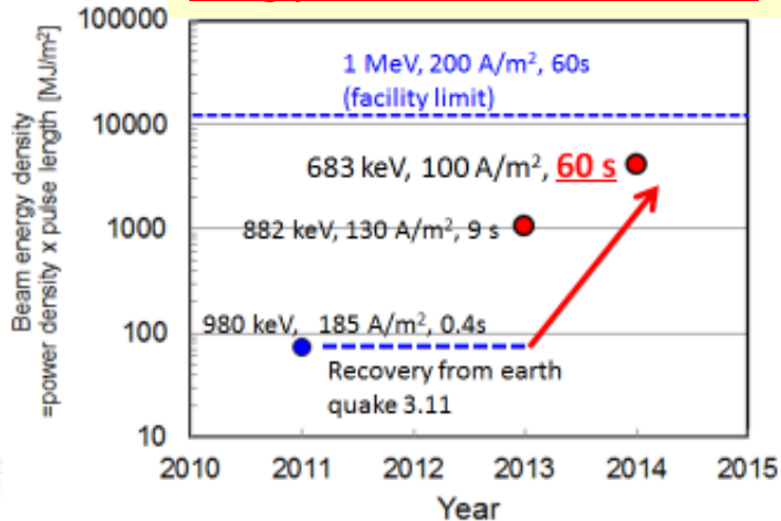
Long pulse beam acceleration
