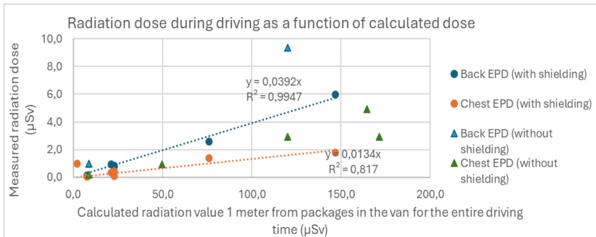
Figure 33: Radiation dose during driving as a function of calculated dose
