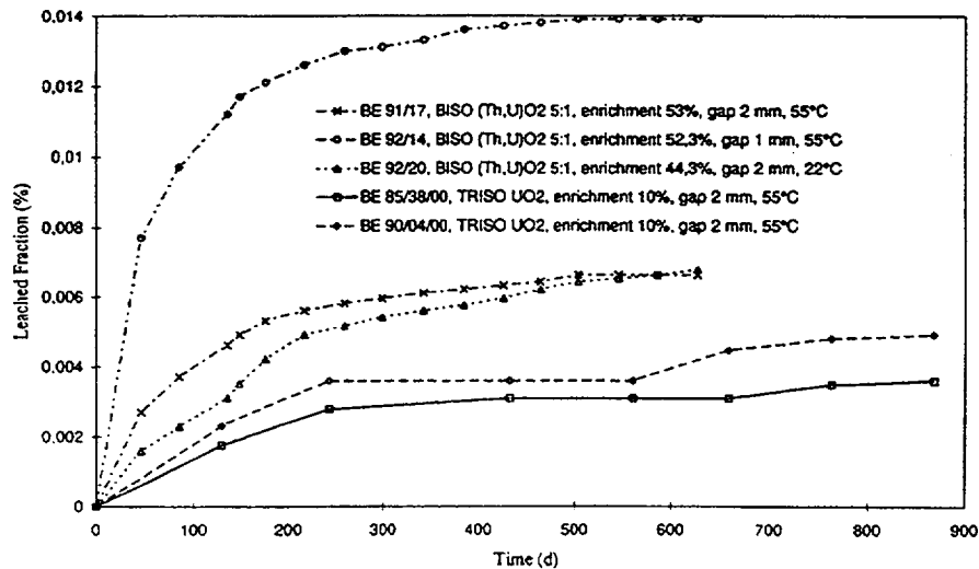
Fig. 19: Fractional release of organic ^{14}\text{C}
