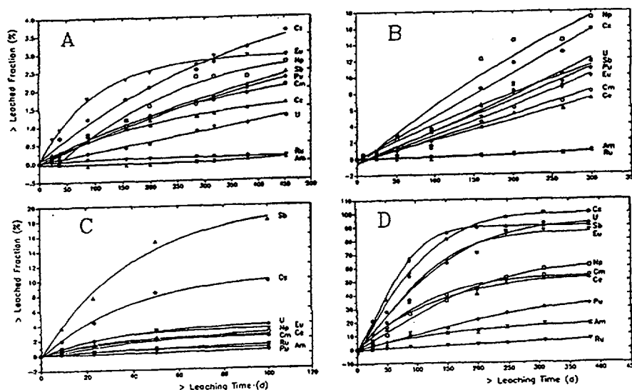
FIG. 13: Radionuclide leaching from \text{UO}_2 kernel with Q-Brine A: 20^\circ\text{C}/100 \text{ kPa} B: 20^\circ\text{C}/13 \text{ MPa} C: 90^\circ\text{C}/100 \text{ kPa} D: 90^\circ\text{C}/13 \text{ MPa}
