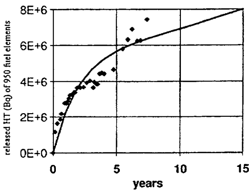
FIG. 3: Release of ^3\text{H}
