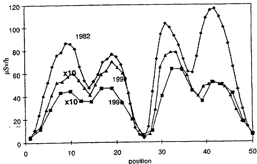
FIG. 8: Gamma dose rate of AVR storage casks
