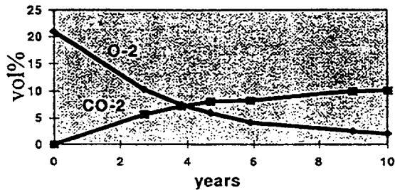
FIG. 6: Gas composition within a storage can
