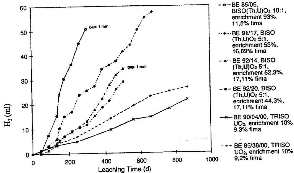
FIG. 18: Hydrogen build-up
