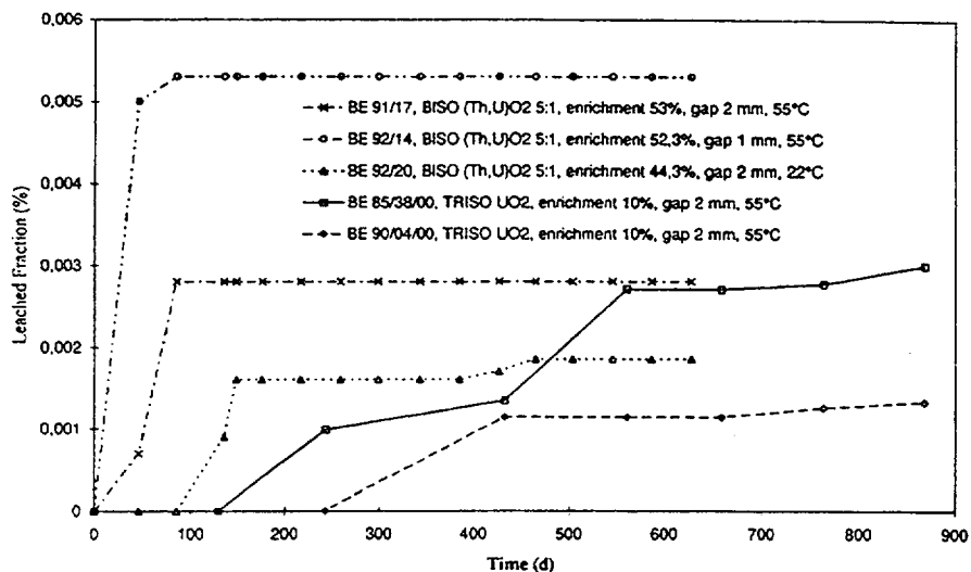
Fig. 20: Fractional release of inorganic ^{14}\text{C}
