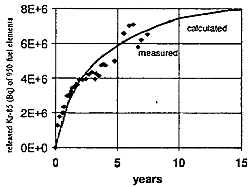
FIG. 4: Release of ^{85}\text{Kr}
