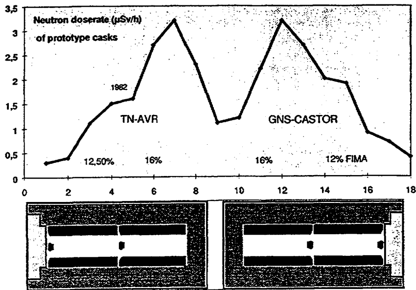
FIG. 9: Neutron dose rate of AVR storage casks
