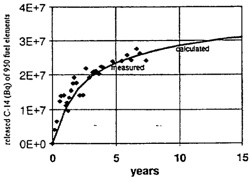
FIG. 5: Release of ^{14}\text{C}
