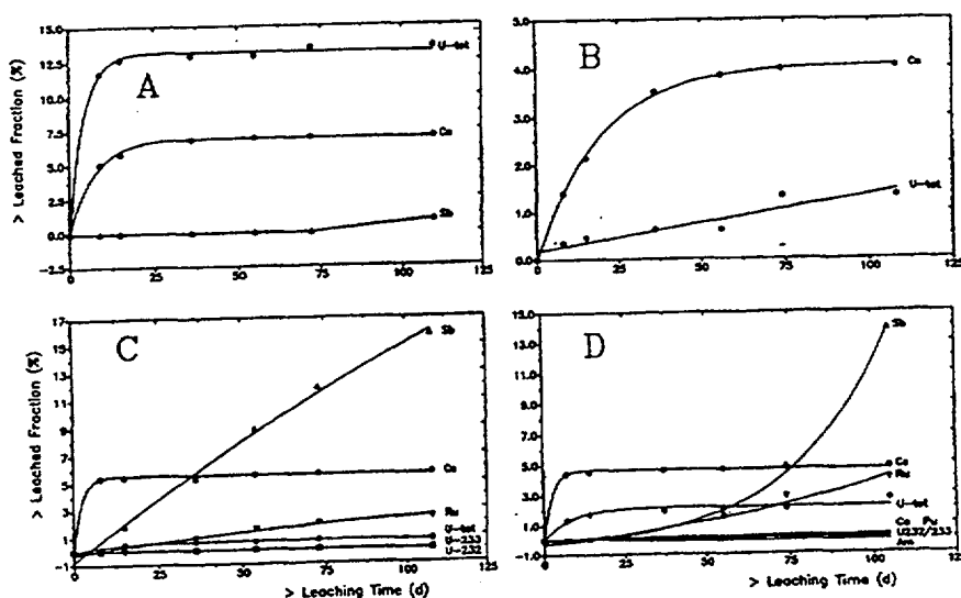
FIG. 14: Radionuclide leaching from (\text{Th,U})\text{O}_2 kernel with Q-Brine A: 20^\circ\text{C}/100 \text{ kPa} B: 20^\circ\text{C}/13 \text{ MPa} C: 90^\circ\text{C}/100 \text{ kPa} D: 90^\circ\text{C}/13 \text{ MPa}
