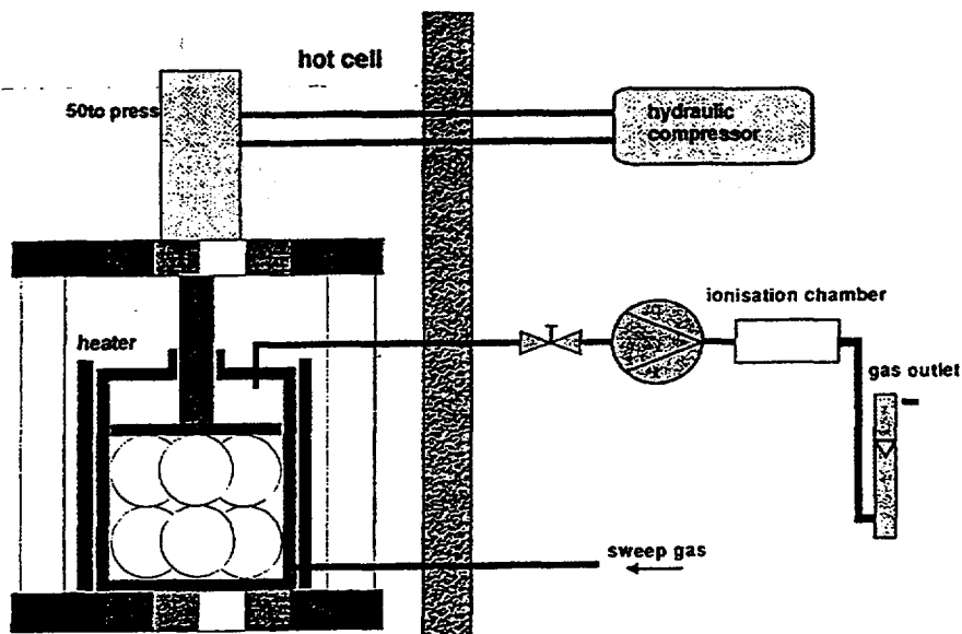
FIG. 10: 50-ton press to crush up to 9 spherical fuel elements (simulation of a mechanical pressure of 30 MPa)
