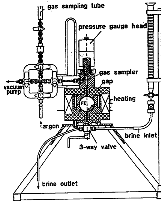
FIG. 17: Spherical autoclave
