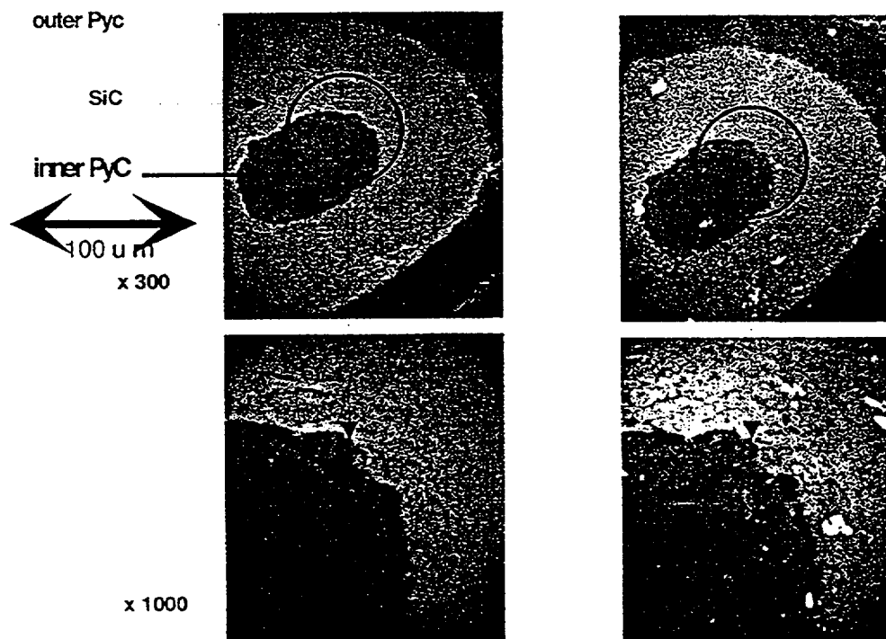
FIG. 16: SEM micrographs of a polished TRISO particle at the beginning (left) of leaching and after 2 years (right).
