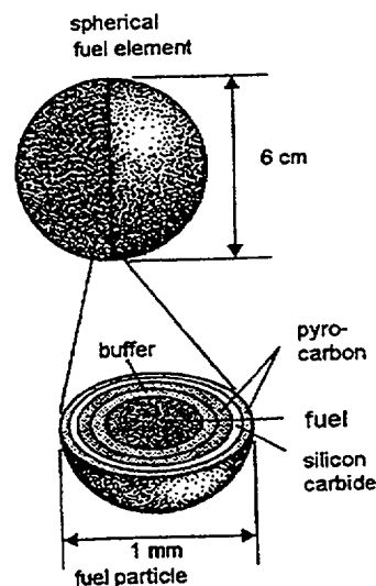
FIG. 1: Sectional view of a HTR fuel element
