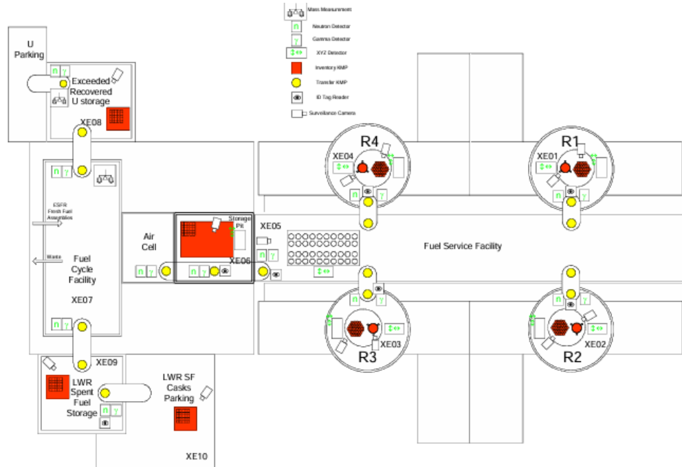
Fig.9. Safeguards system developed for the Example Sodium Fast Reactor (ESFR), object of the GIF PRPP case Study.
