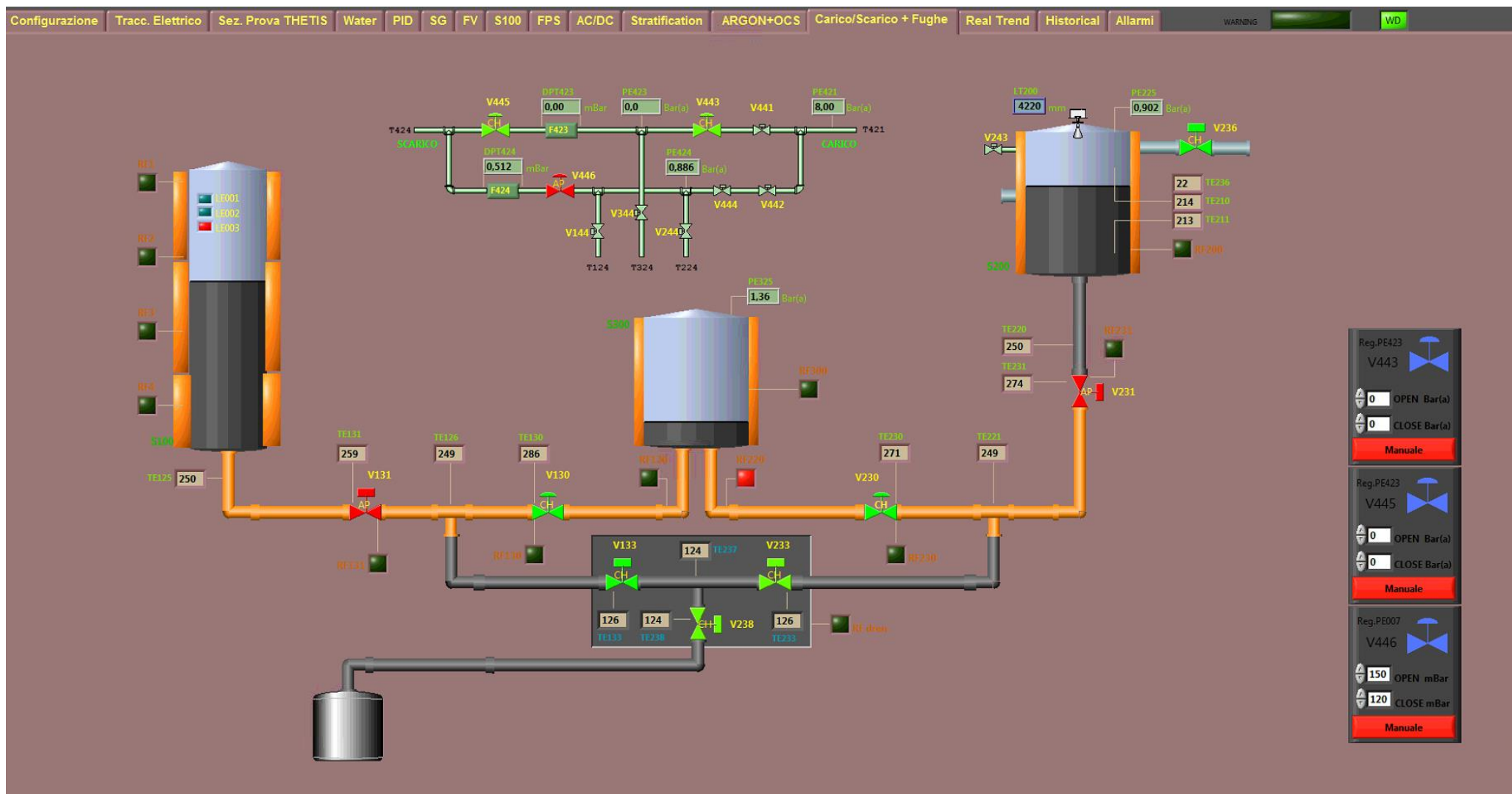
CIRCE-THETIS SCADA view – Fill&Drain control panel
