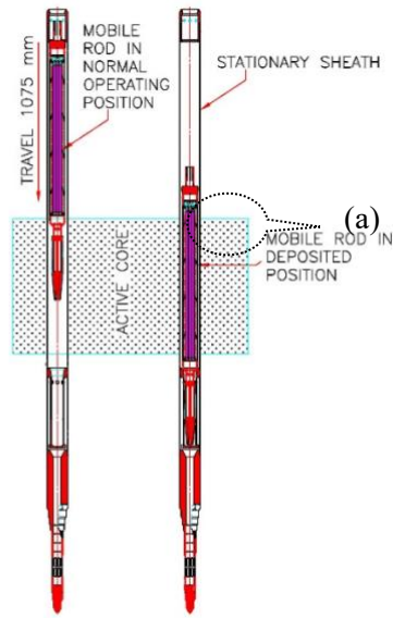
(a) Seating interface of mobile rod and seat FIG. 1. Schematic of HSAR while dropped condition and suspended condition
