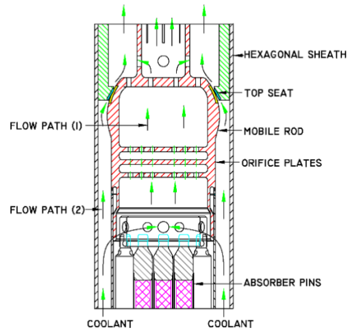
(a) Seating interface of mobile rod and seat FIG. 1. Schematic of HSAR while dropped condition and suspended condition
