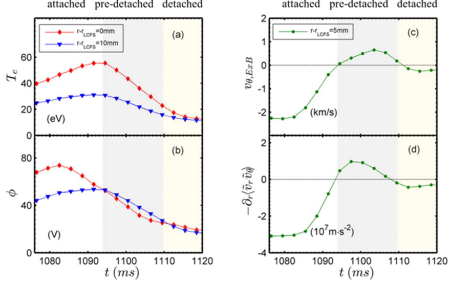
FIG. 3. (a) Temperature, (b) potential, (c) E \times B poloidal velocity and (d) Reynolds force during the divertor detachment
