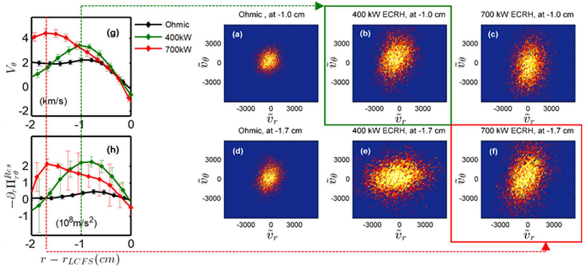
FIG. 1. (a)(b)(c) Joint PDF of radial and poloidal velocity fluctuations at 1.0 cm inside LCFS; (d)(e)(f) joint PDF of radial and poloidal velocity fluctuations at 1.7 cm inside LCFS; (g) E \times B poloidal flow; (h) intrinsic poloidal torque, in Ohmic and 400/700 kW ECRH heated discharges.
