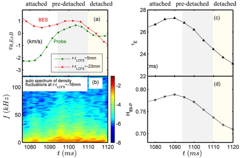
FIG. 4. (a) Edge E \times B poloidal velocity shear, (b) time-frequency auto-spectrum of density fluctuations, (c) plasma energy confinement time and (d) energy confinement enhanced factor during the divertor detachment
