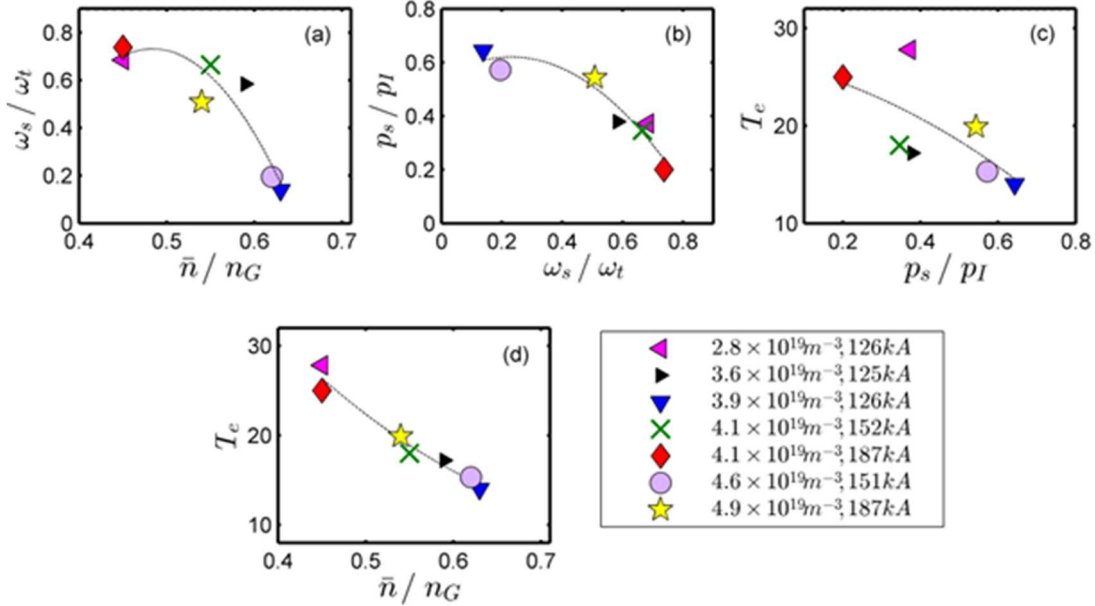
FIG. 2. (a) The normalized E \times B shearing rate \omega_N = \omega_s/\omega_t VS the Greenwald fraction f_G = \bar{n}/n_G ; (b) the normalized turbulence spreading power \mathcal{P}_N = \mathcal{P}_S/\mathcal{P}_I VS the normalized E \times B shearing rate \omega_N = \omega_s/\omega_t ; (c) the edge electron temperature VS the normalized turbulence spreading power \mathcal{P}_N = \mathcal{P}_S/\mathcal{P}_I ; (d) the edge electron temperature VS the Greenwald fraction f_G = \bar{n}/n_G
