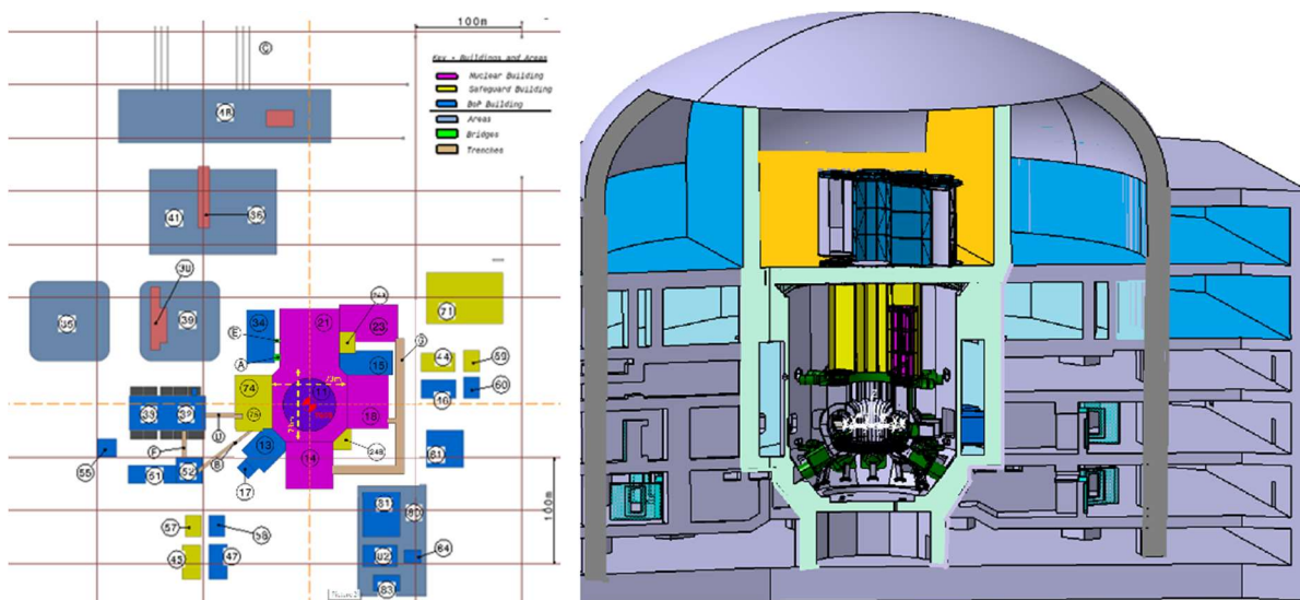
FIG. 2. Left: VNS site with arrangement of nuclear buildings, buildings hosting tokamak auxiliary systems, and power supply and heat rejection installations, right: section of the left side of the tokamak building.
