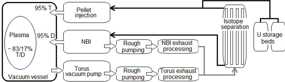
FIG. 3. Block diagram of basic VNS D-T fuel cycle.
