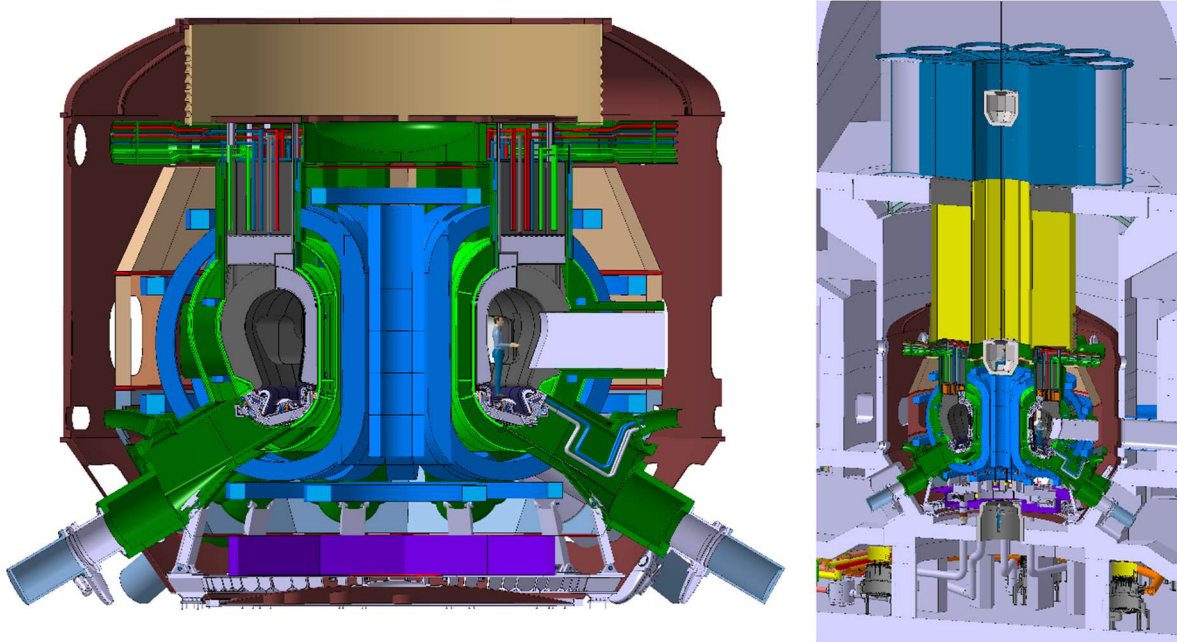
FIG. 1. Left: VNS tokamak, Right: personnel access to the joints of the magnet coils via shielding cabins to the central upper and lower areas of the cryostat
