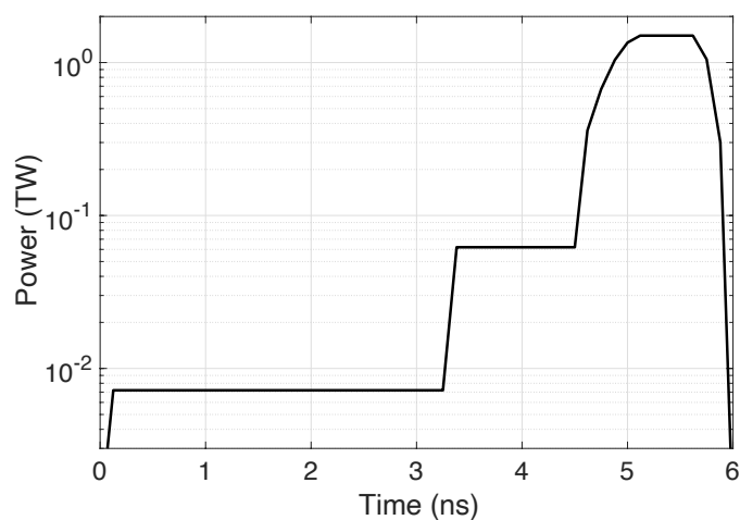
Fig.1 Laser waveform used in experiment which was optimized by 1-D radiation hydrodynamics simulation code to maximize the areal density.
