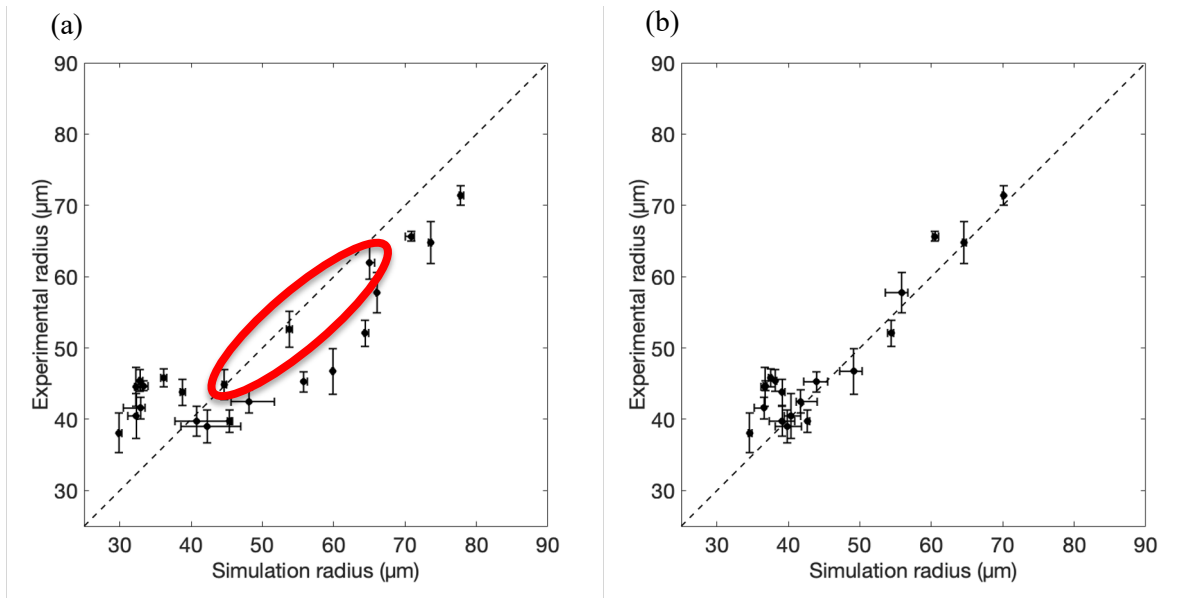
Fig.2 Comparison of the experimental and simulation results (a). The comparison trends differ between the cases with little glue (b) Input parameters on the simulation is artificially adjusted.
