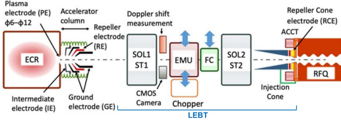
FIG. 1. Configuration of LIPAc Injector
