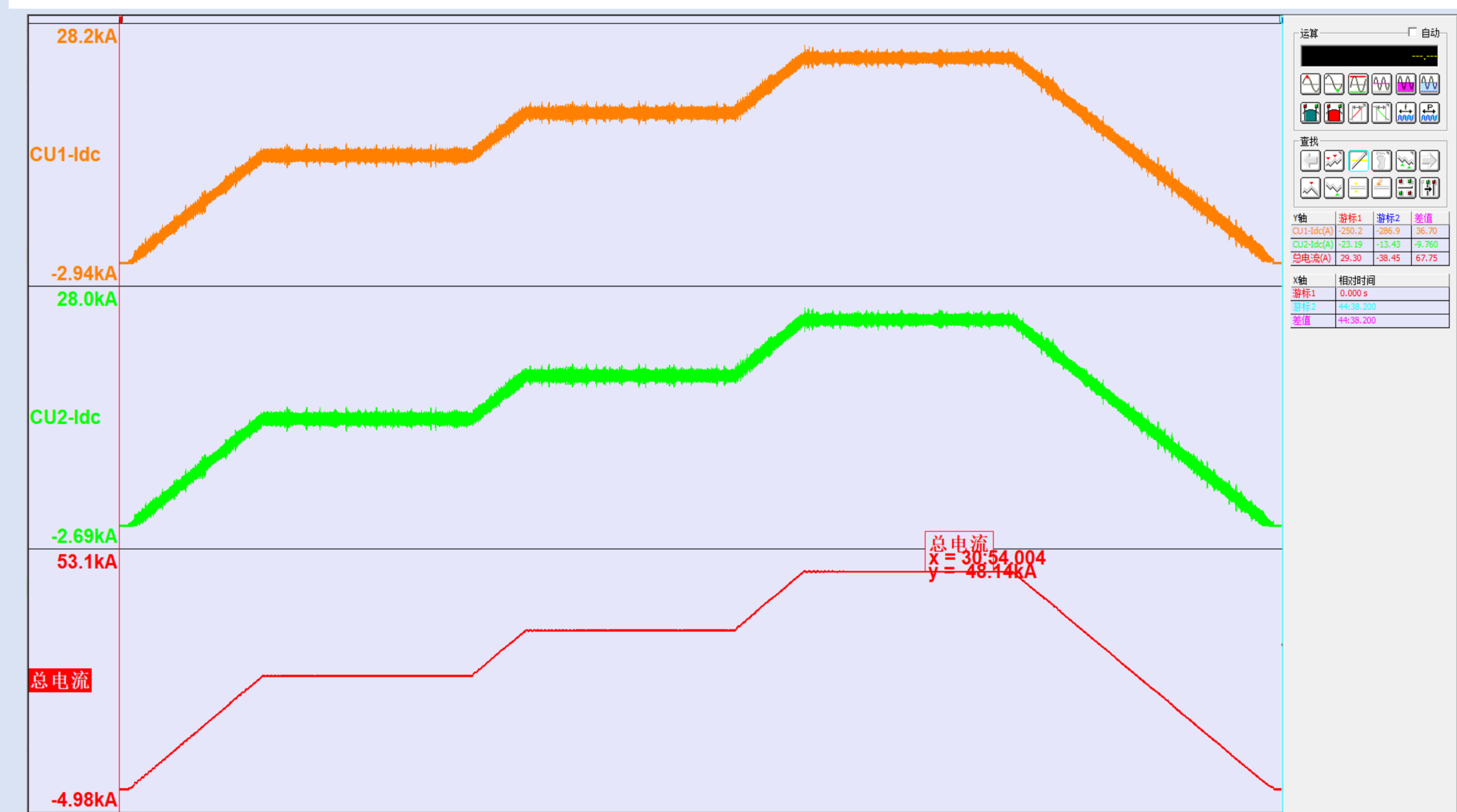
Figure 4. 48 kA True Load Current Waveform
