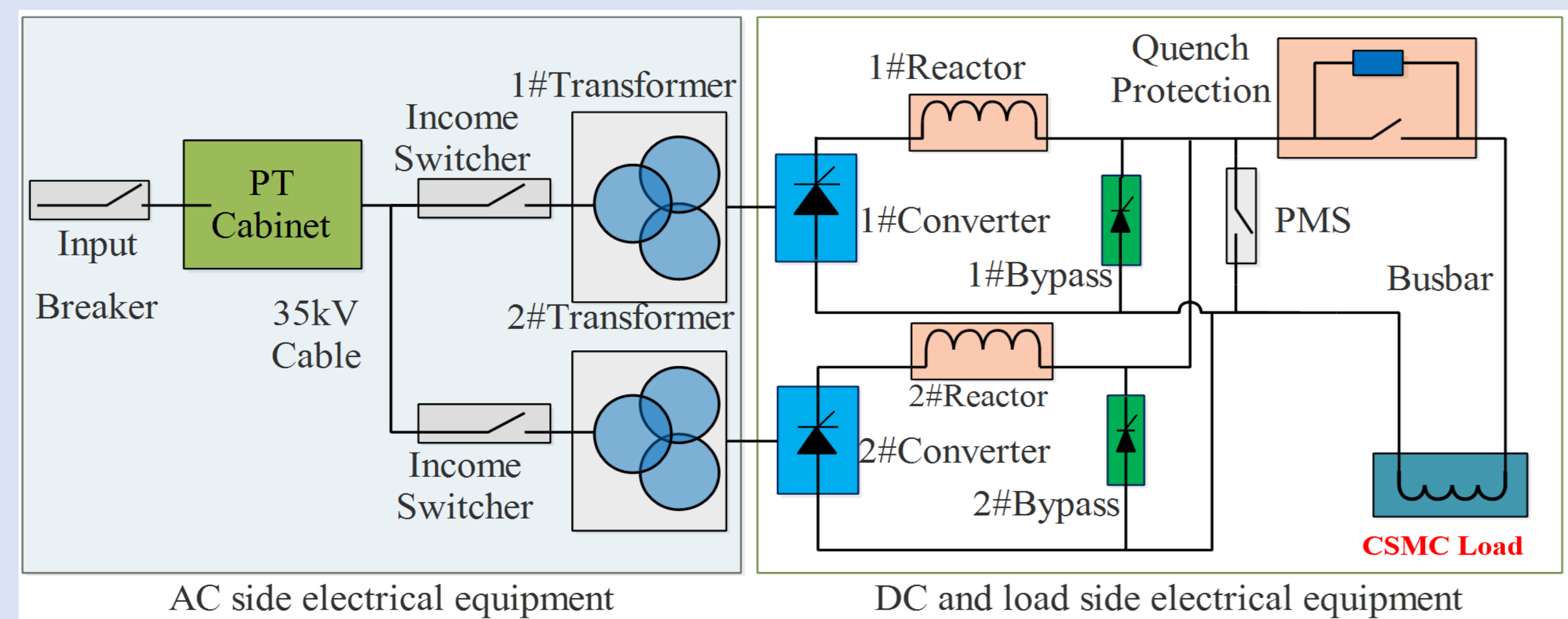
Figure 3. Topological Diagram of Electrical Equipment
