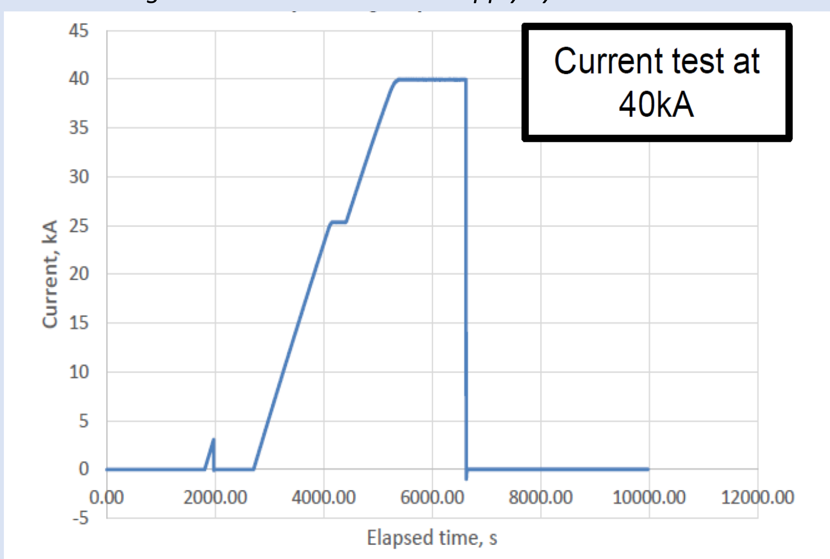
Figure 2. ITER CSMC Test Current Waveform
