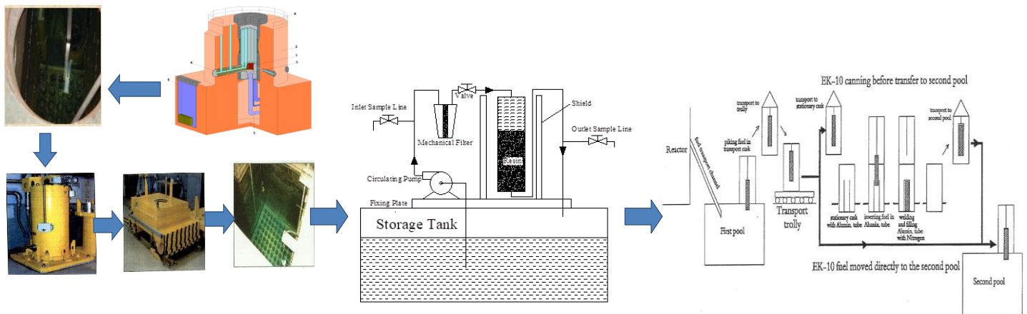
Fig. 1 Defueling, Ion Exchange and SF Encapsulation Process in ETRR-1
