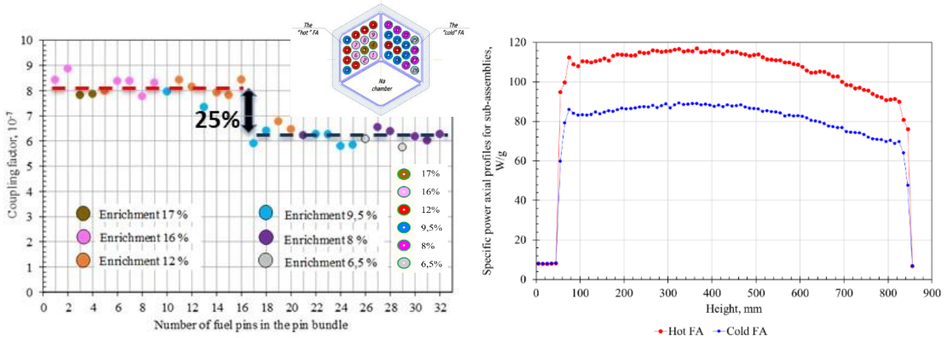
FIG. 4 : Fuel pin configuration according to their enrichment in ^{235}\text{U} in the two Fuel sub-Assemblies (FA) : pin to pin (on the left) and axial profile (on the right)
