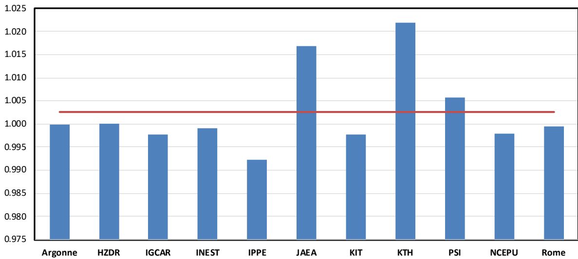
FIG. 4. Neutron Multiplication Factor and Average (Red Line)
