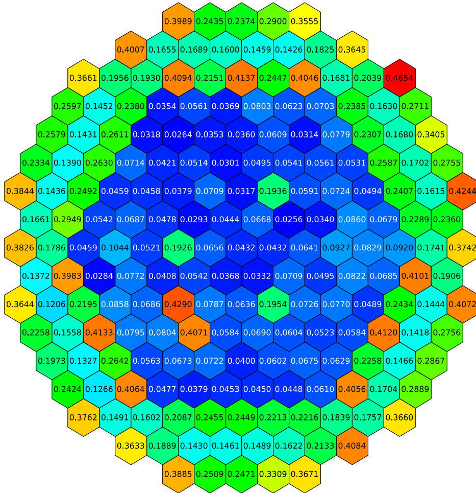
FIG. 2. Variation in Radial Power Profile Results (Standard Dev. / Average)
