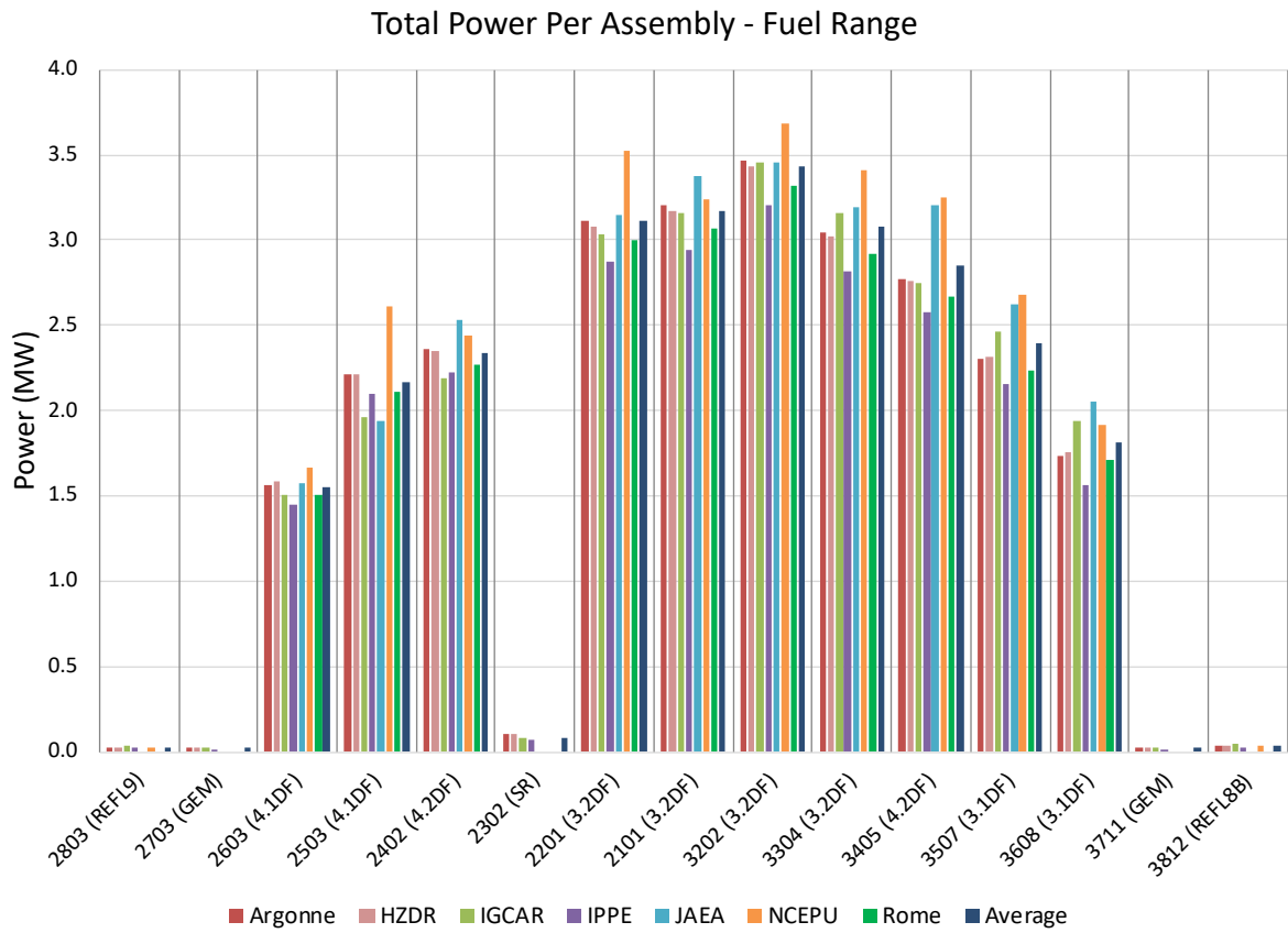
FIG. 3. Variation in Radial Power Profile In Several Assemblies
