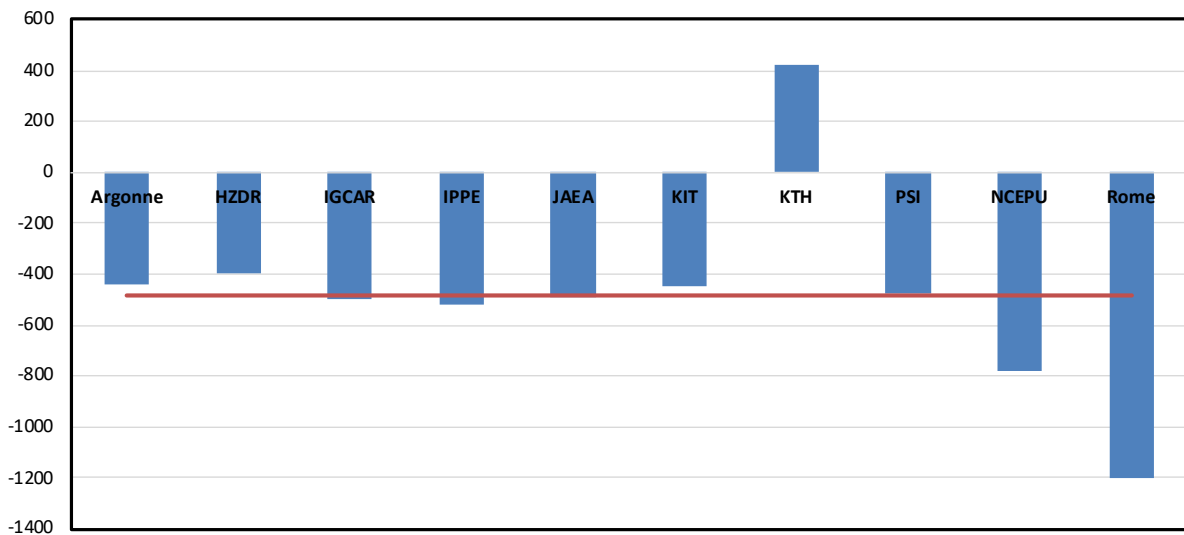
FIG. 6. Blind Results – Gas Expansion Modules (pcm) Worth and Average (Red Line)
