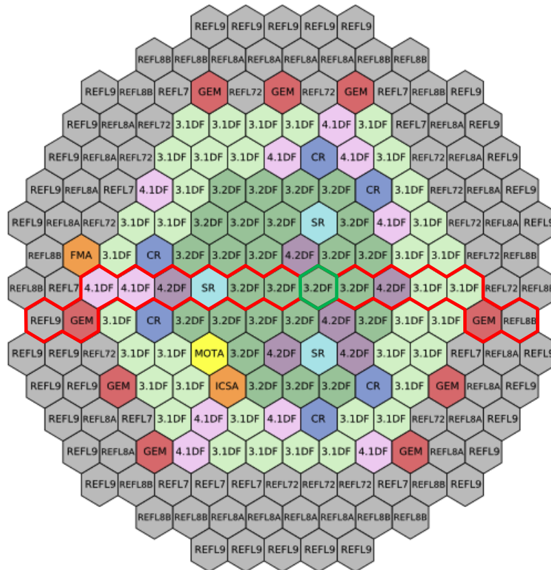
FIG. 1. Radial layout of FFTF core
