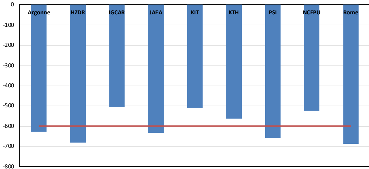
FIG. 5. Fuel Doppler Constant (pcm) and Average (Red Line)
