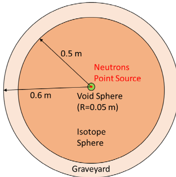
Figure 2.1 – Sphere Leakage benchmark geometry
