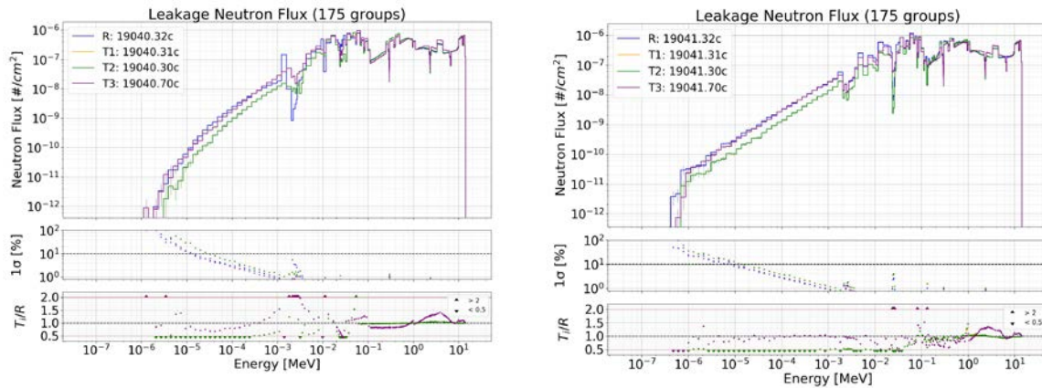
Figure 3.2 – Neutron leakage flux comparison between FENDL v3.2, FENDL v3.1, FENDL v3.0 and ENDF-VII.1 for the Potassium-40 (left) and Potassium-41 (right)
