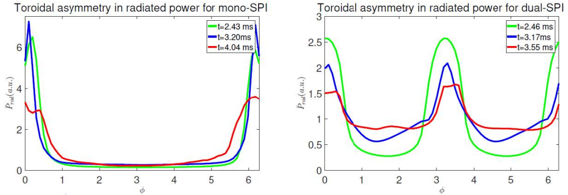
Figure 1: Toroidal distribution of the radiated power (normalized to the toroidally averaged radiated power) from a JOEKE simulation of Ne+D2 SPI into an ITER plasma, either from a single injector (left) or from two toroidally opposite and perfectly synchronized injectors (right). The green and blue curves correspond to the pre-TQ, while the red curves are right after the TQ.
