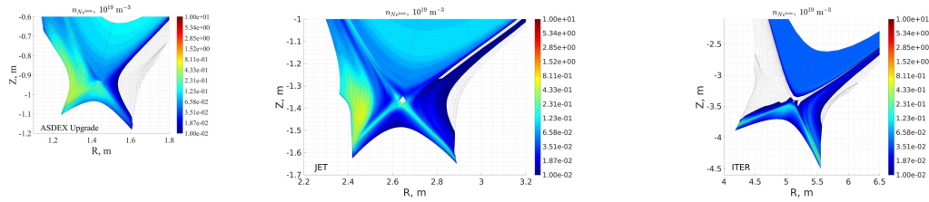
Figure 2: SOLPS-ITER neon ions density(all charge states) distributions for all 3 machines.
