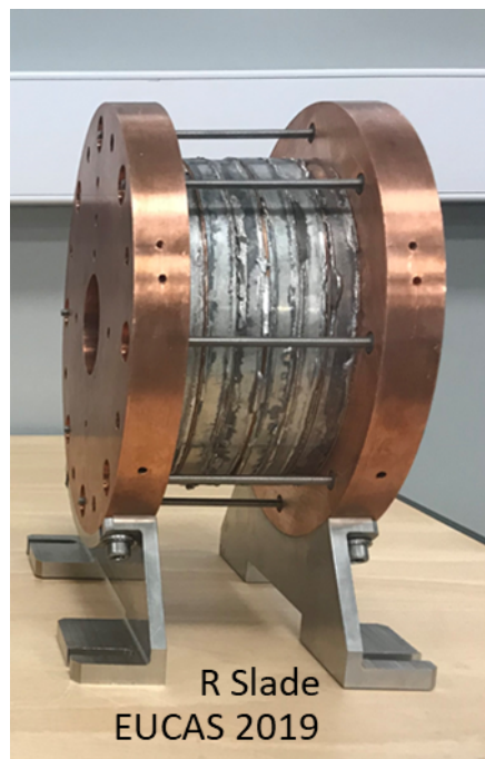
Figure 3: 24.4T HTS test coil
