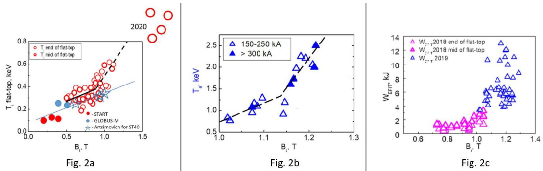
Figure 2: Sharp increase in T_i , T_e and WEFIT at TF >1 – 1.1 T), which may suggest transition to a better confinement at higher TF.
