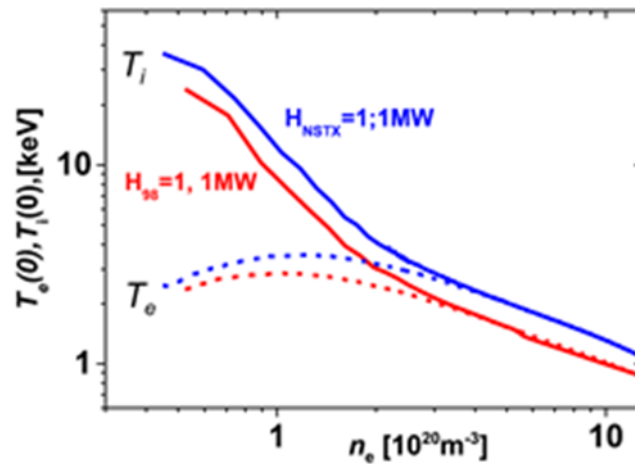
Figure 4: T_i , T_e vs line averaged density with 1MW absorbed power, ASTRA simulations
