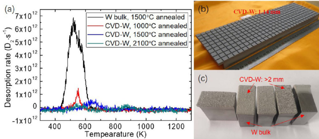
Figure 2: (a) TDS results of the pure W bulk and CVD-W samples after annealing at temperatures in the range of 1000-2100 °C for 1 h, (b) Large-scale deposition of CVD-W on the CuCrZr alloy, (c) W bulk samples with CVD-W coatings for the manufacture of water-cooled monoblocks.
