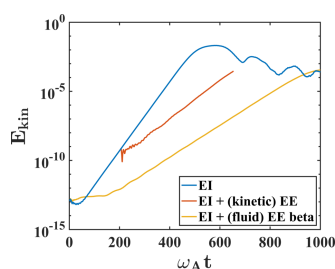
Figure 6: Kinetic energy evolution of energetic ion (EI) driven TAE with the effect of energetic electrons (EEs).
