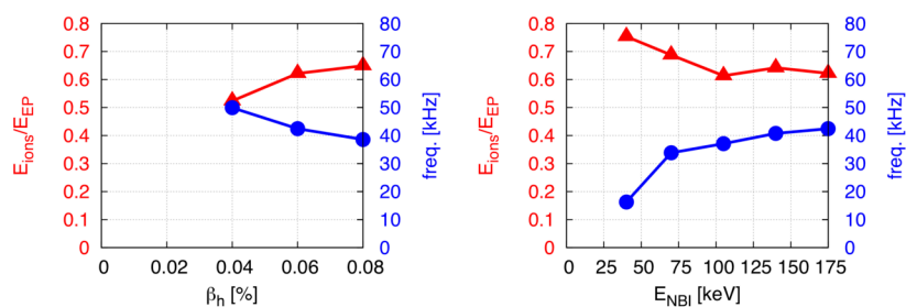
Figure 8: The energy transfer efficiency (triangles) and EGAM frequency (circles) versus the energetic particle pressure (left panel) and beam energy (right panel).
