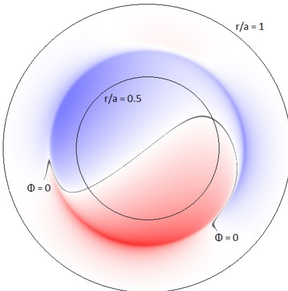
Figure 1: poloidal mode structure
