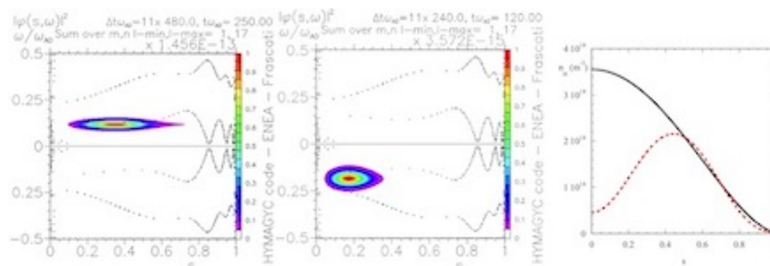
Figure 7: NLED-AUG case, n=1 : (left) frequency spectrum for the electrostatic potential and monotonic EP density profile (black solid curve, see the right frame), and (centre) frequency spectrum for nonmonotonic EP density profile (red dashed curve, see the right frame); Maxwellian EP distribution function with temperature TH=0.093 MeV.
