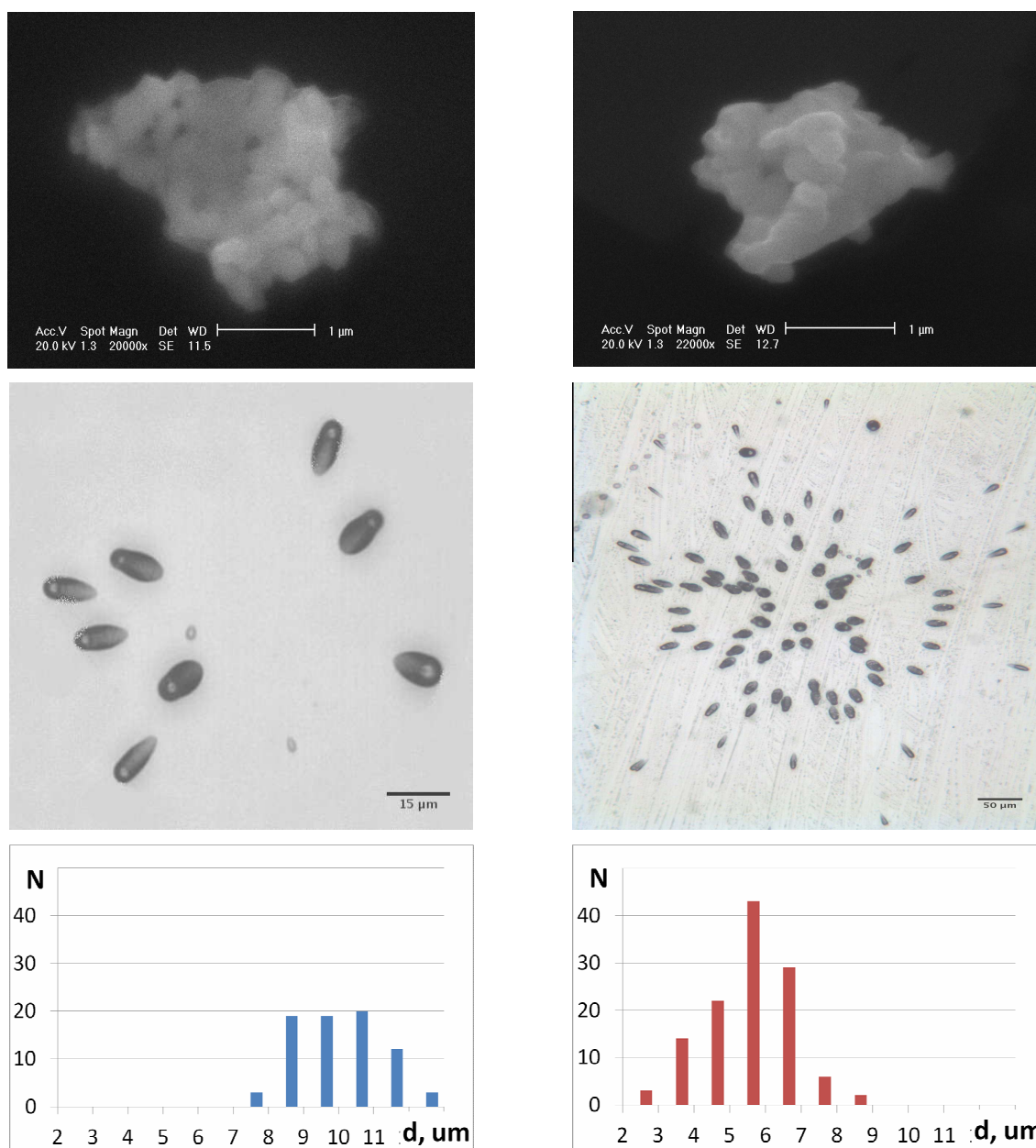
FIG. 2. Uranium (left) and plutonium (right) particles, corresponding alpha-track clusters and histograms of tracks distribution on values d for 4 uranium particles (blue) and 2 plutonium particles (red).
