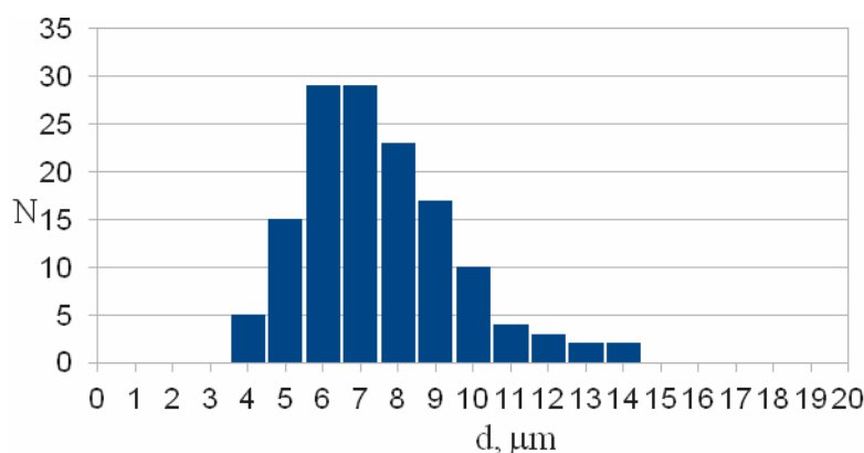
FIG. 5. Size distribution of diameter d for fragment 1 (particle 1).
