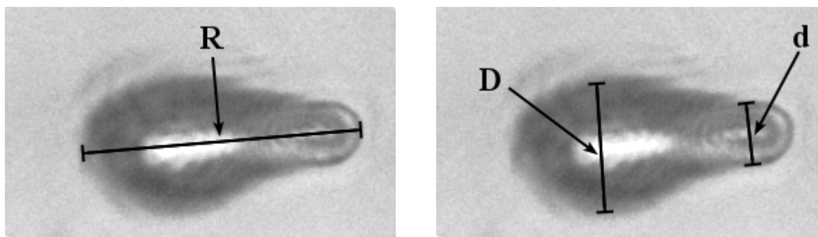
FIG. 1. Characteristics of individual alpha-track: length (large axis) R , diameter D of the input hole, diameter d of the curvature of cone top of the track.
